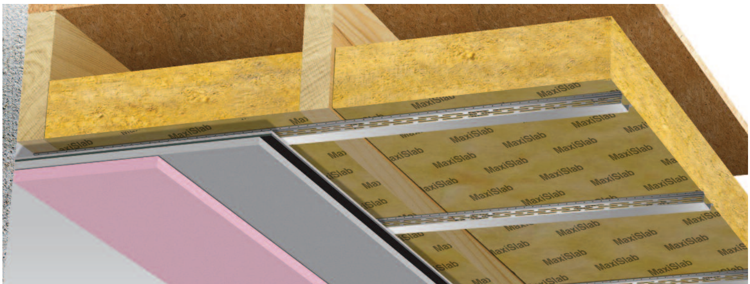
Maxi 60 Ceiling – shiplap edge detail.
